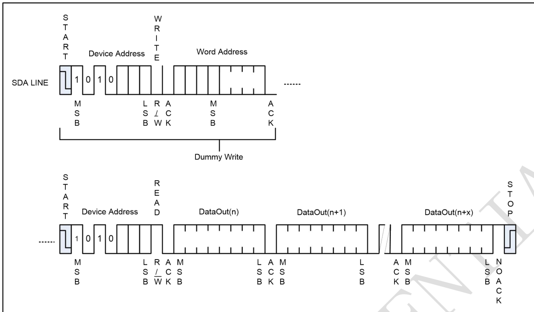
Figure 5-5 Sequential Read
