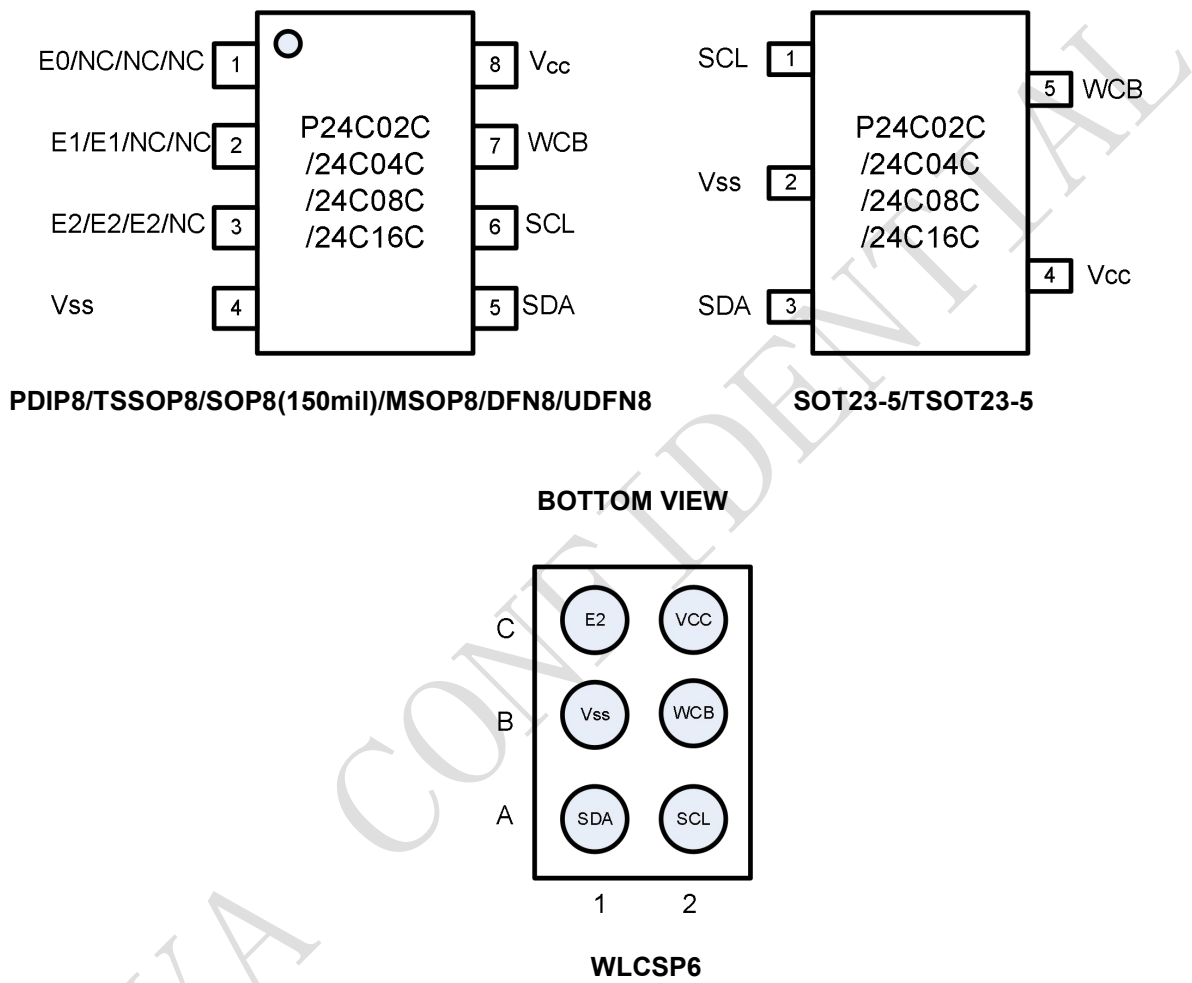
Figure 1-1 Pin Configuration
